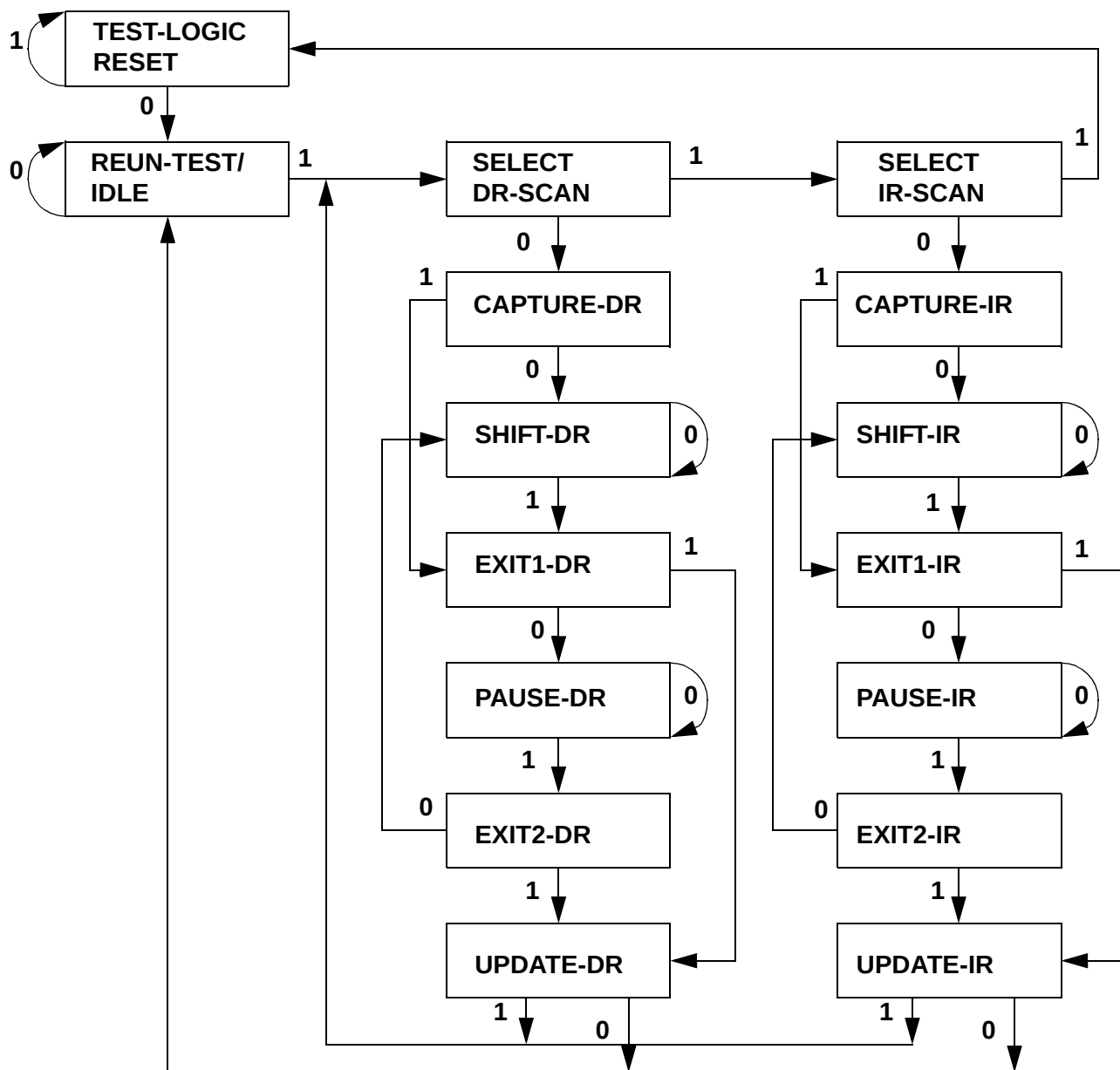
Figure 1. TAP Controller State Diagram [13]
