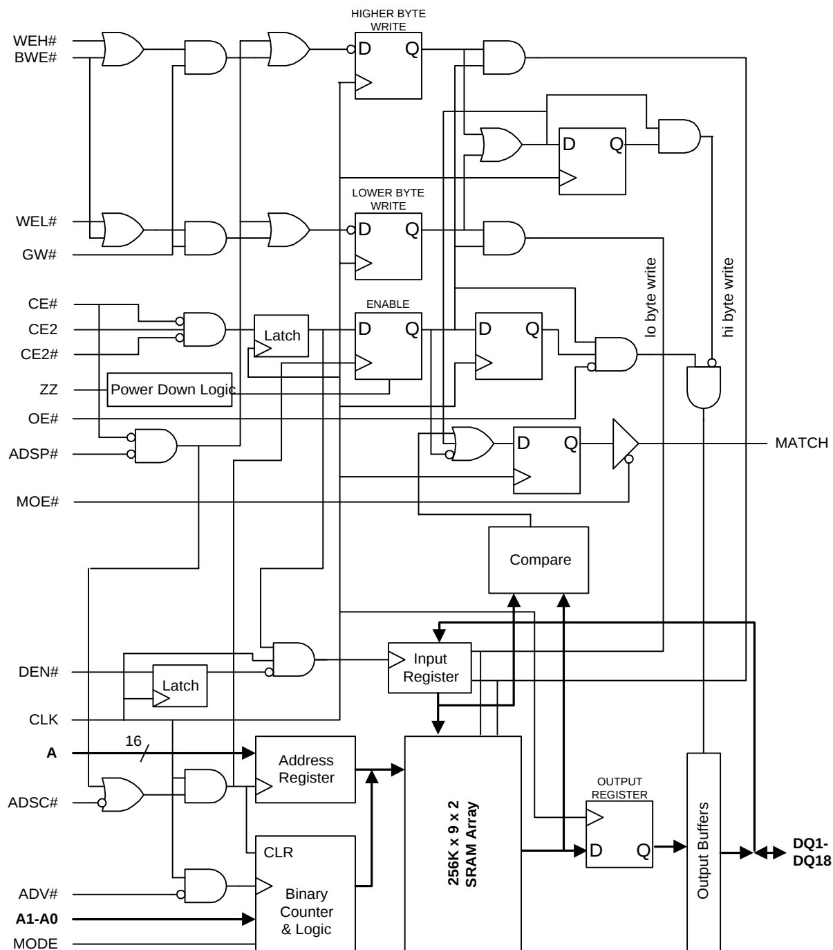
Functional Block Diagram—256Kx18 [1]
