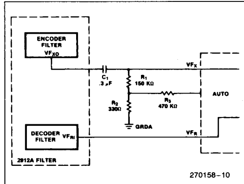
Figure 12. Circuit Interface—With External Auto Zero
