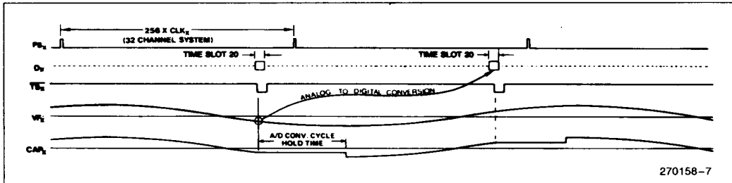
Figure 7. Transmit Encoding
