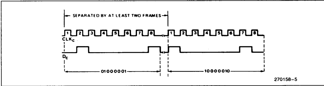
Figure 5. Microcomputer Mode Programming Examples
