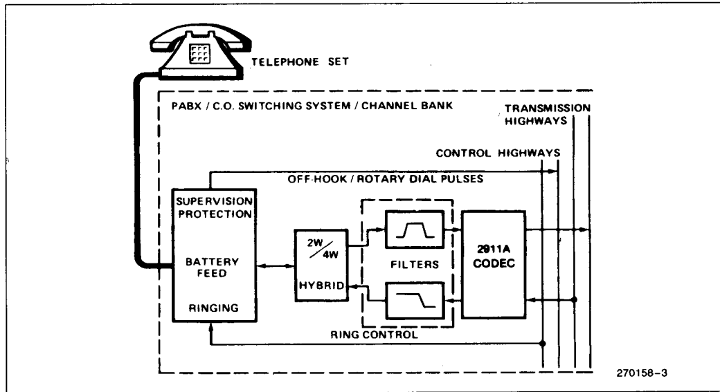
Figure 4. Typical Line Termination
