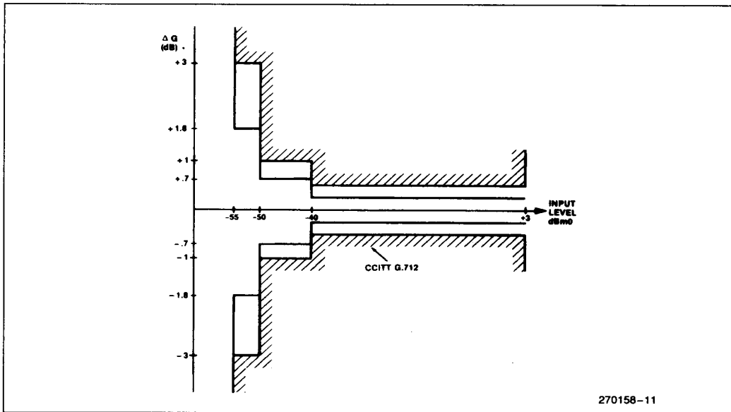
Figure 13. Tracking Deviation ( \Delta G ) (Half Channel)
