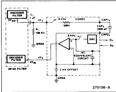
Figure 11. Circuit Interface—Without External Auto Zero
