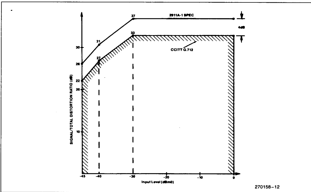
Figure 14. Signal to Total Distortion Ratio (Half Channel)
