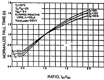
SWITCHING TIME VS. BASE CURRENT (TYPICAL)
