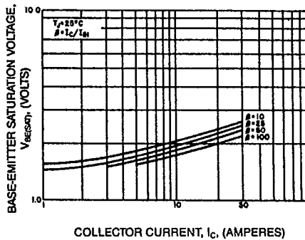
SATURATION VOLTAGE (TYPICAL)
