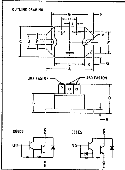
500-600-700 Volts D66DS, D66ES Outline Drawing
