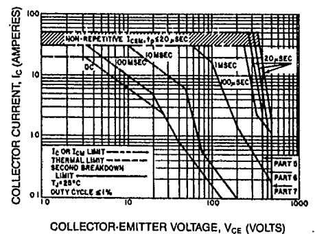
FORWARD BIAS SAFE OPERATING AREA (S.O.A.)
