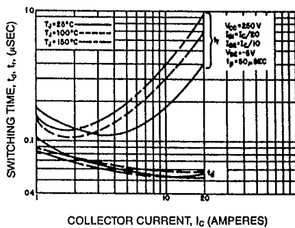
SWITCHING CHARACTERISTICS (TYPICAL)
