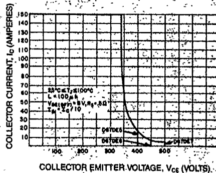
REVERSE BIAS SAFE OPERATING AREA (R.B.S.O.A.)
