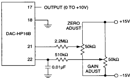
Figure 3. Unipolar Operations
