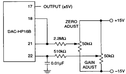
Figure 4. Bipolar Operations
