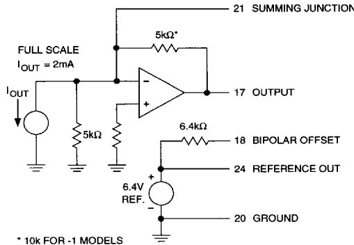
Figure 5. Output Circuit
