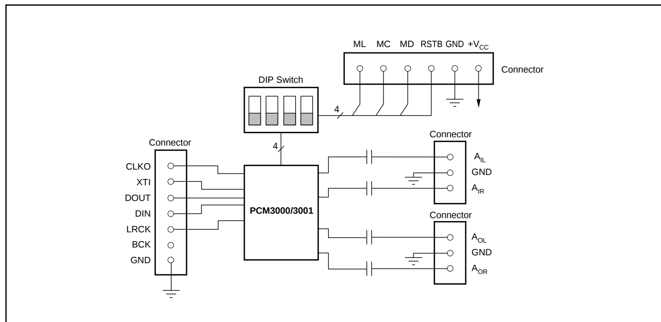
FIGURE 1. DEM-PCM3000/3001 Block Diagram.
