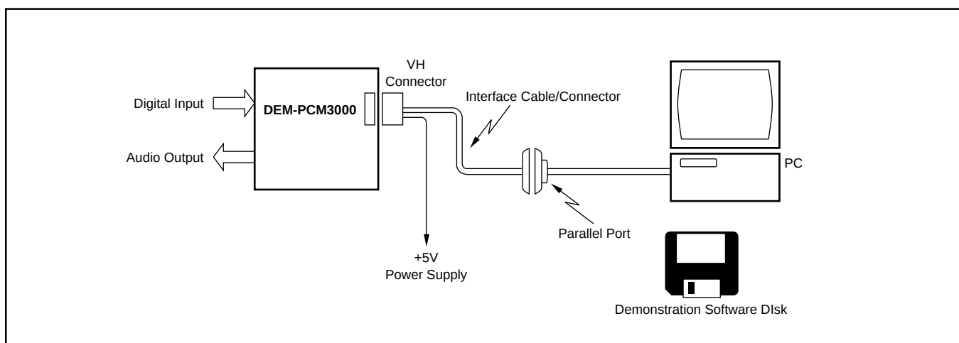
FIGURE 5. DEM-PCM3000-1 Interface Connection.
