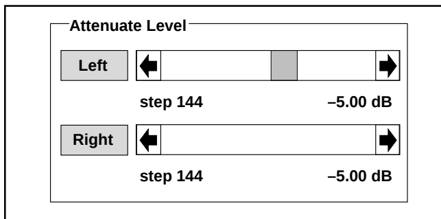
FIGURE 9. PCM3000 Attenuate Control for Simultaneous Channels.
