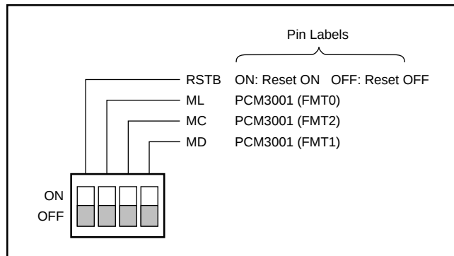
FIGURE 2. Format and Reset Control.
