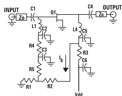
Figure 8. Passive Biasing.
