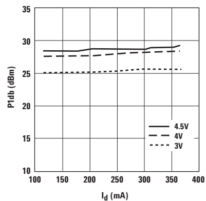
Figure 29. P1dB vs. I_{ds} and V_{ds} at 3.9 GHz.
