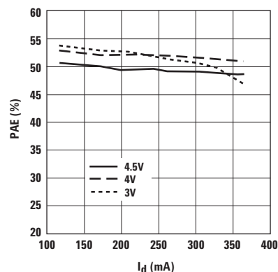
Figure 33. PAE @ P1dB vs. I_{ds} and V_{ds} at 2 GHz.
