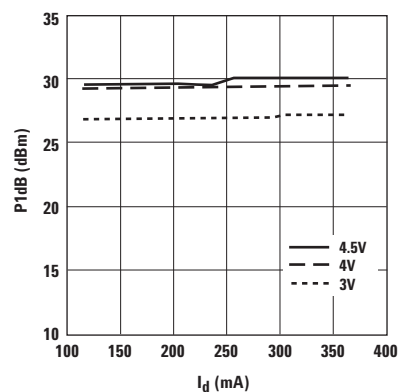
Figure 27. P1dB vs. I_{ds} and V_{ds} at 2 GHz.
