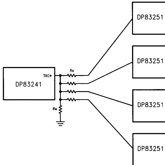
FIGURE 5-7. CDD Device Driving Four PLAYER Devices in Parallel
