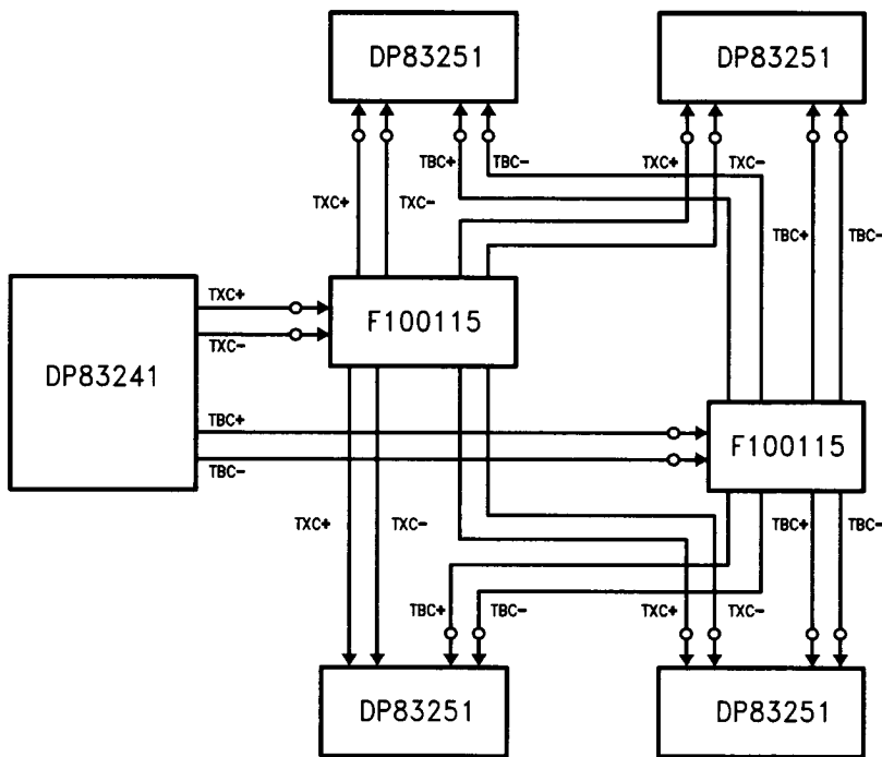
FIGURE 5-9. CDD Device Driving Four PLAYER Devices Using Two F100115 Quad Low Skew Drivers
