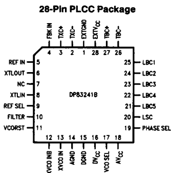
FIGURE 2-1. DP83241 Pinout
