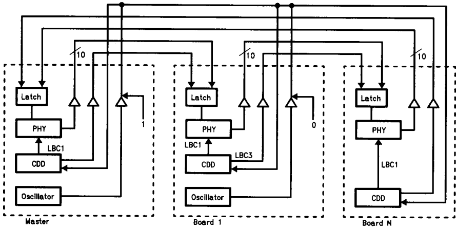
FIGURE 5-4. Large Concentrator Application
