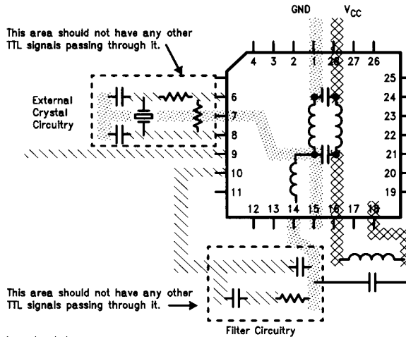
FIGURE 5-10. Recommended Layout
