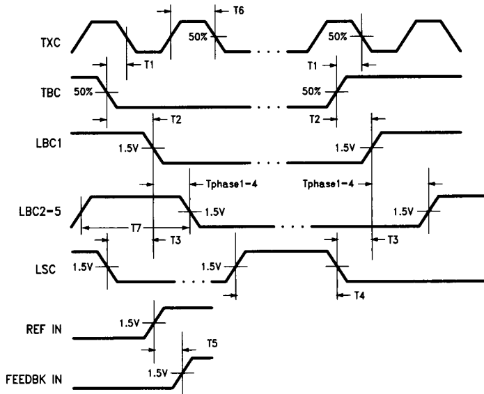
FIGURE 4-1. AC Timing Waveforms
