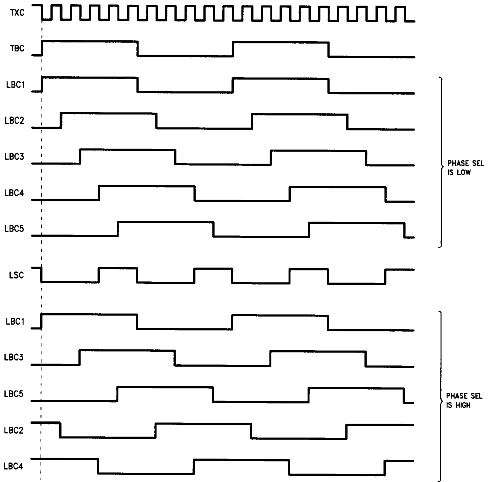
FIGURE 4-2. Typical Clock Relationships
