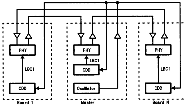
FIGURE 5-3. Small Concentrator Application
