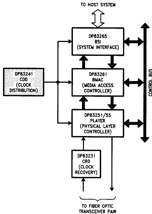
FIGURE 1-1. FDDI Chip Set Block Diagram
