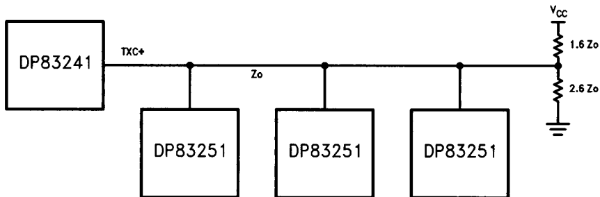
FIGURE 5-8. Proper Bus Line Termination and Connections
