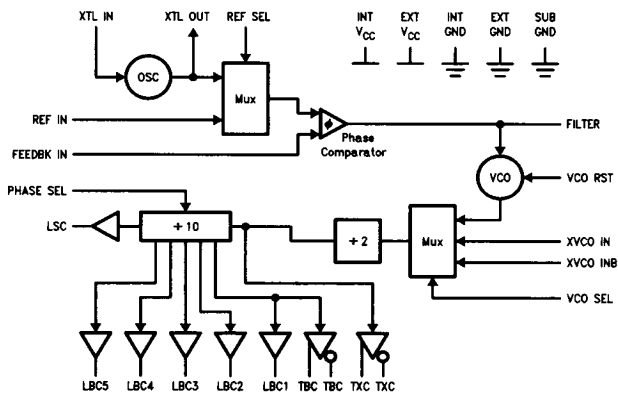
FIGURE 2-2. DP83241 Block Diagram
