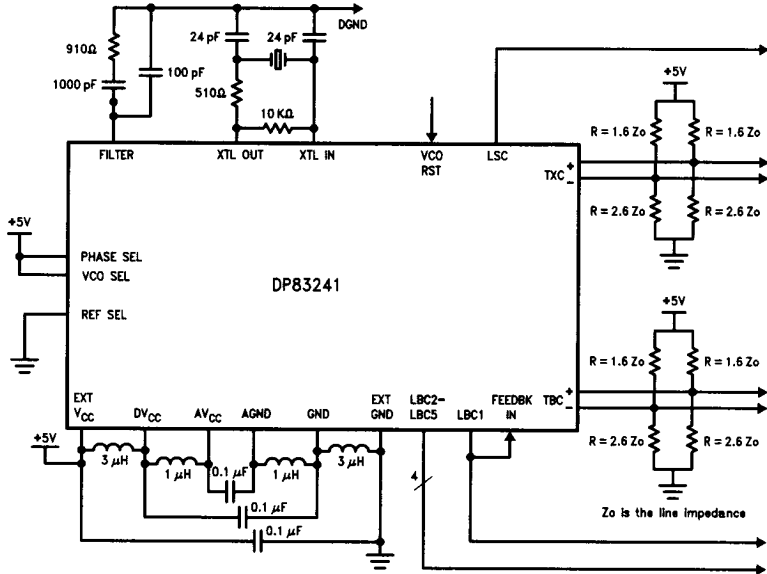
The Filter components are based on a 12.5 MHz Crystal and a 250 MHz VCO. All component values \pm 10\% .
