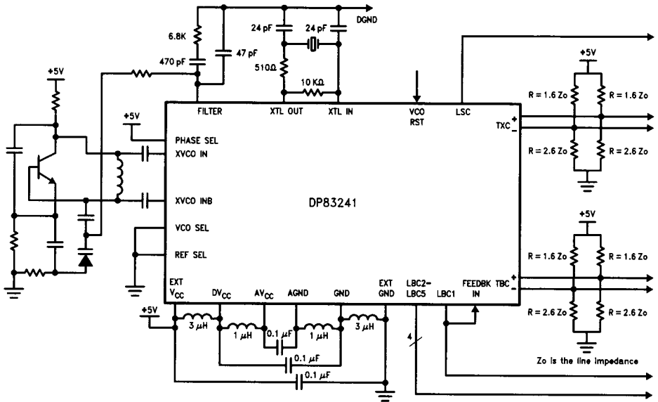
The Filter components are based on a 12.5 MHz Crystal and an external 250 MHz VCO with a gain of 40 MRad/V. All component values \pm 10\% .
