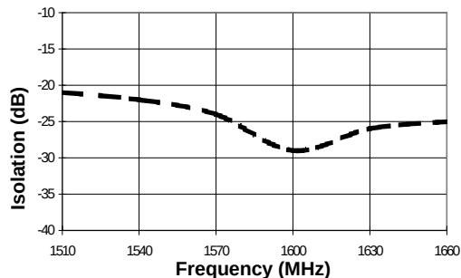
Isolation vs Frequency
