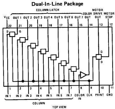
Order Number DS8693N See NS Package N22A
