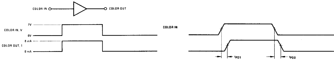
FIGURE 4. DS8693 Color Driver
