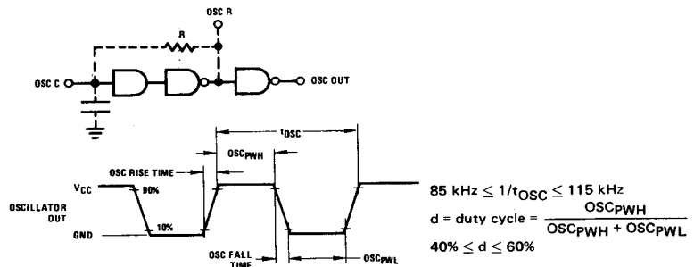
FIGURE 7. DS8694 Oscillator Diagram
