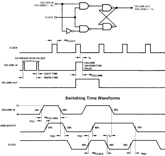
FIGURE 3. DS8693, DS8694 Column Latch
