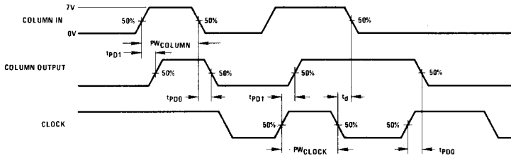
FIGURE 3. DS8693, DS8694 Column Latch
