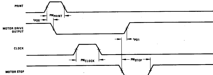
FIGURE 6. DS8693 Motor Drive Latch
