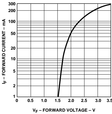
Figure 9. Forward Current vs. Forward Voltage.
