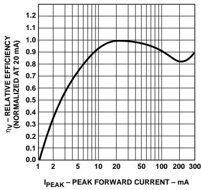
Figure 11. Relative Efficiency vs. Peak Forward Current.
