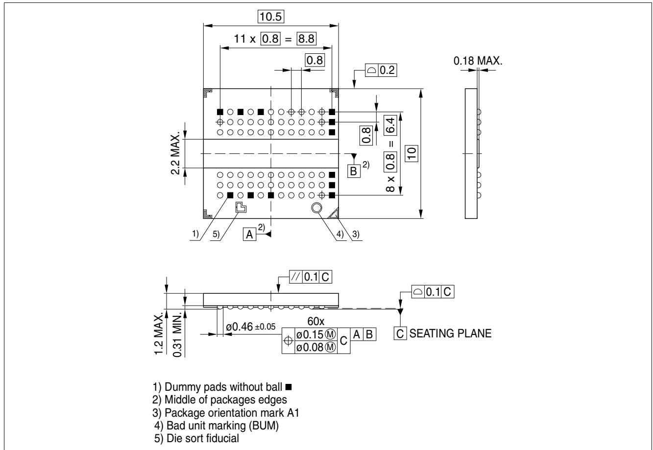
Figure 78 Package Pinout PG-TFBGA-60 (bottom view)
