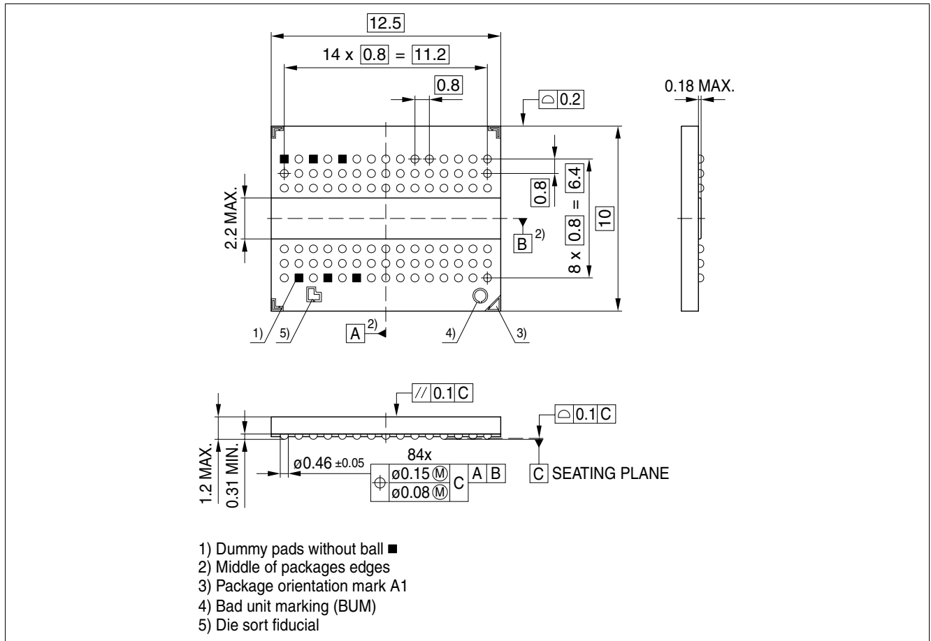
Figure 79 Package Pinout PG-TFBGA-84 (bottom view)
