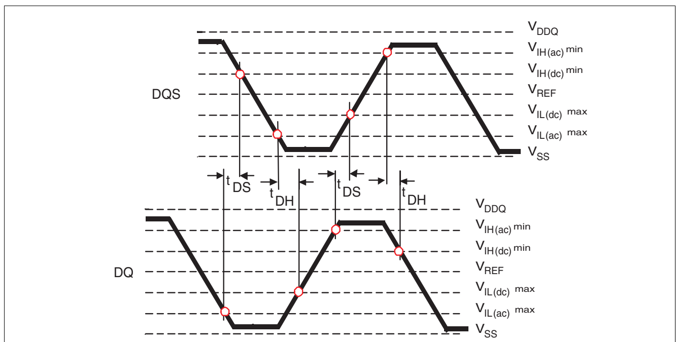
Figure 75 Data Setup and Hold Time (Single Ended Data Strokes)
