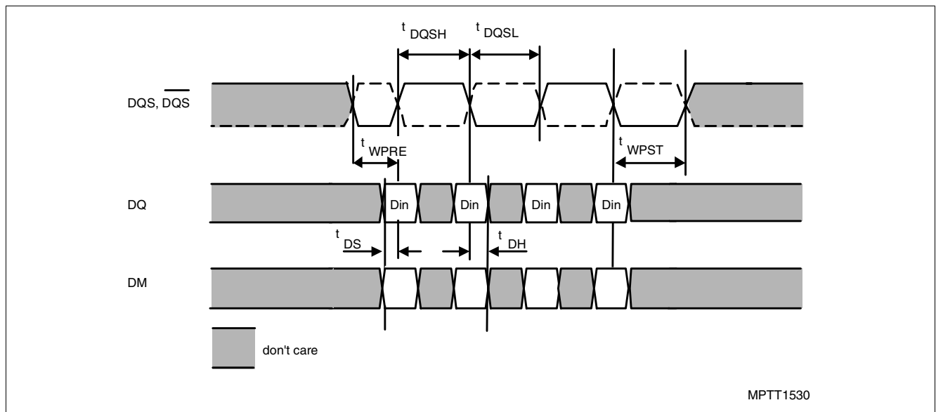
Figure 36 Write Data Mask Timing
