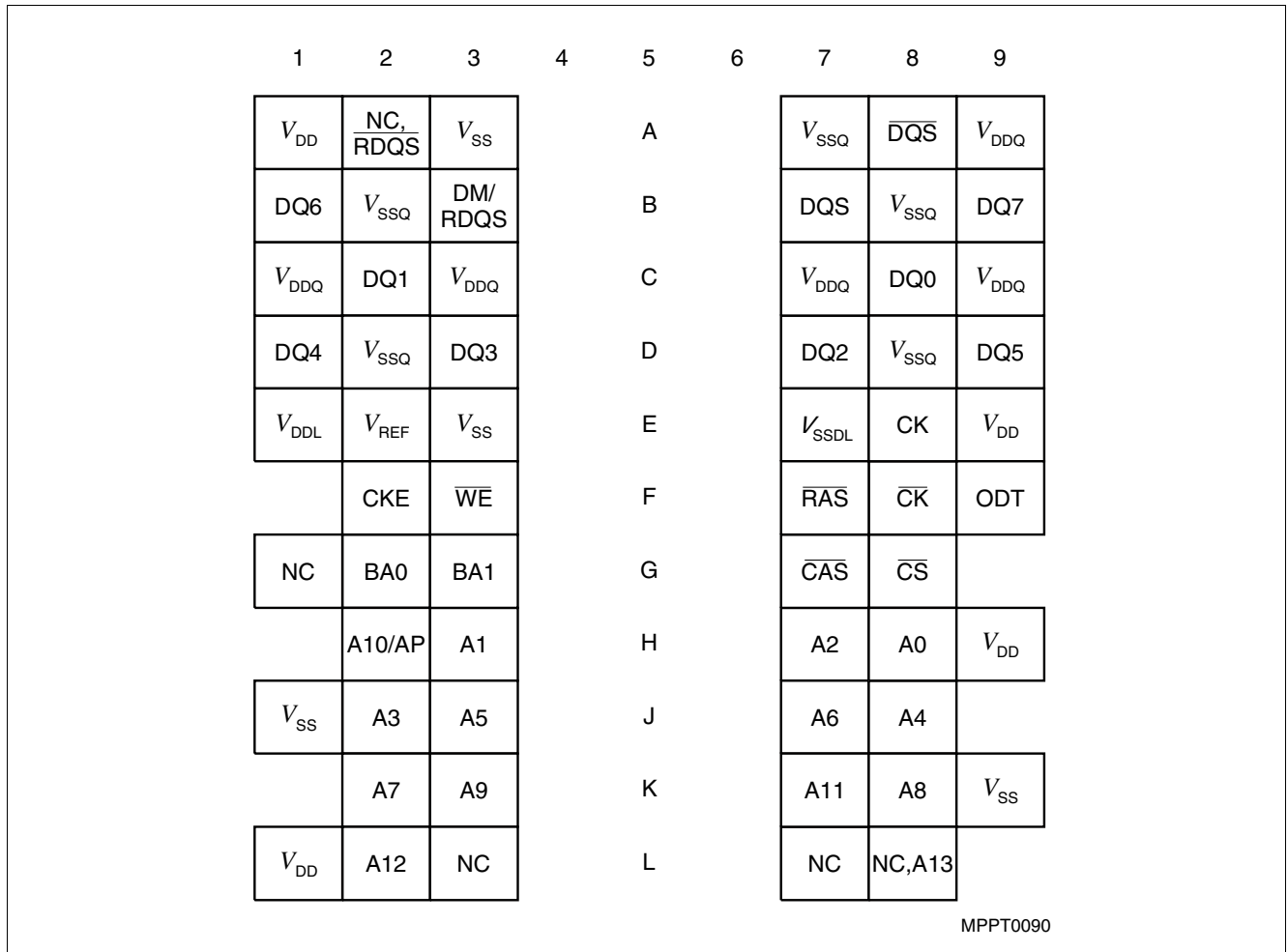
Figure 2 Pin Configuration for ×8 components, PG-TFBGA-60 (top view)
