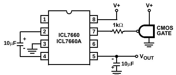
FIGURE 17. EXTERNAL CLOCKING
