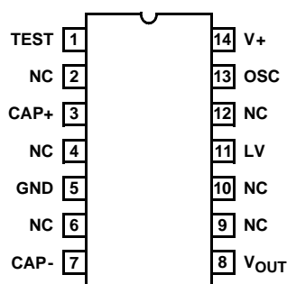
ICL7662CBD-0 (SOIC) TOP VIEW
