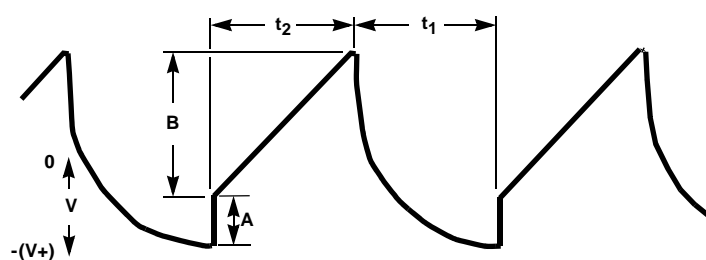
FIGURE 17. OUTPUT RIPPLE
