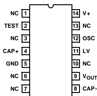
ICL7662CBD AND IBD (SOIC) TOP VIEW
