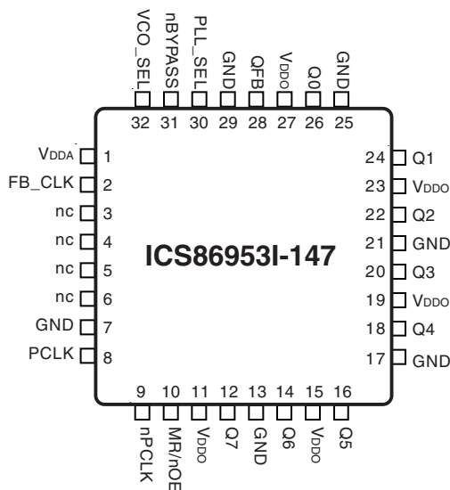
32-Lead LQFP
