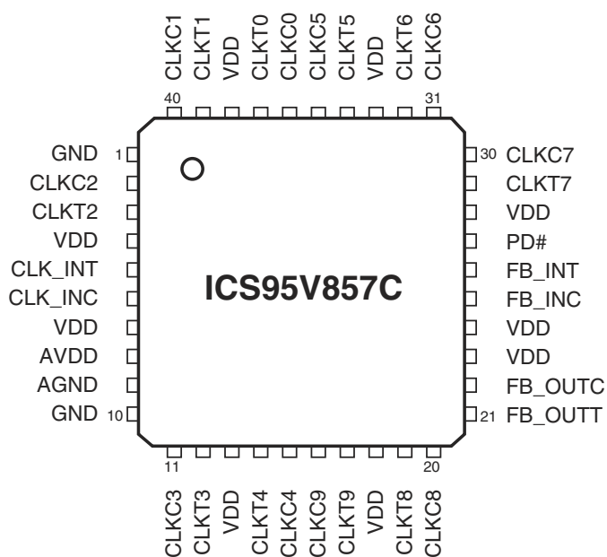
40-Pin MFL
