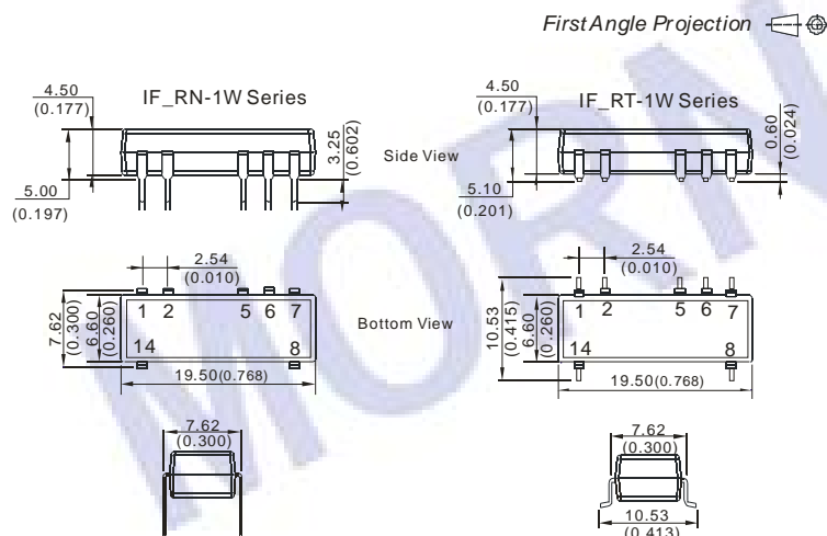
RECOMMENDED FOOTPRINT Top view, grid: 2.54*2.54mm(0.1*0.1inch)
