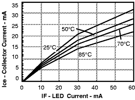
Figure 6. Collector-emitter current versus temperature and LED current
