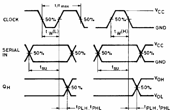
Figure 2. Switching Waveforms
