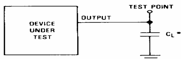
Figure 4. Test Circuit
