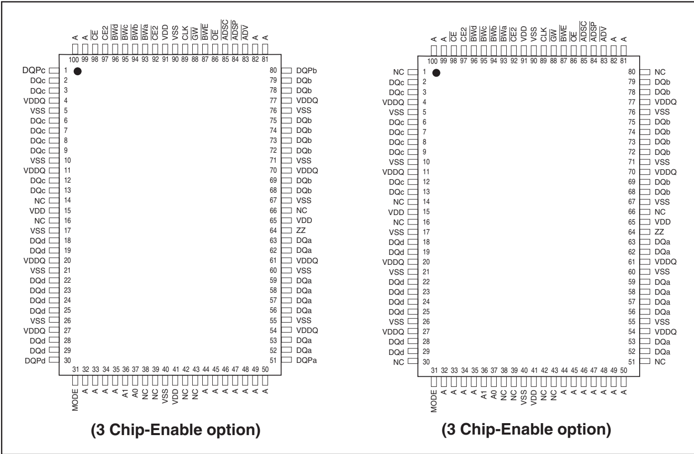
100-PIN TQFP (128K x 36)
