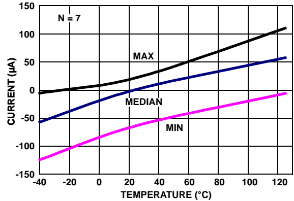
FIGURE 24. ISL28276 SUPPLY CURRENT vs TEMPERATURE, V_+, V_- = \pm 2.5V ENABLED, R_L = INF
