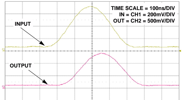
FIGURE 20. 2T RESPONSE
