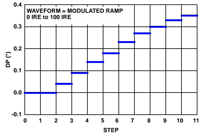
FIGURE 16. DIFFERENTIAL PHASE
