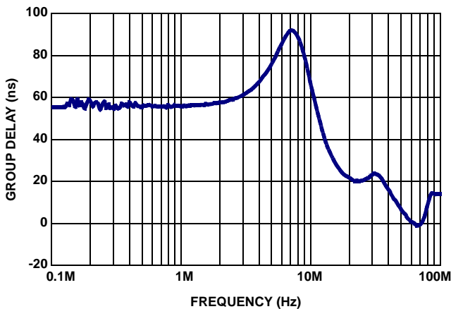
FIGURE 23. GROUP DELAY vs FREQUENCY
