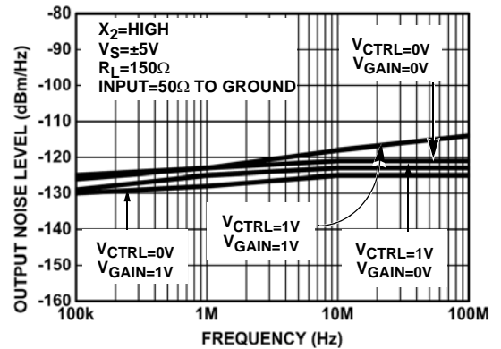
FIGURE 10. OUTPUT NOISE
