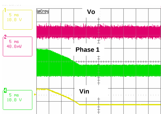
FIGURE 15. 19V TO &gt;8V INPUT LINE TRANSIENT RESPONSE AT ILOAD = 5A AND VID = 1.15V
