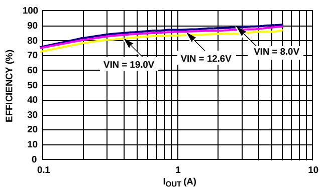
FIGURE 8. EFFICIENCY OF 1-PHASE DE MODE, \text{PSI}_L = \text{LOW} , DCM MODE, \text{VID} = 0.9\text{V} , \text{OFFSET} = 33\text{mV}
