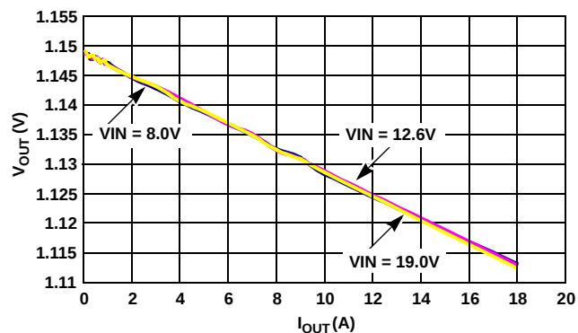
FIGURE 7. ACTIVE MODE LOAD LINE, 1 PHASE, DE, \text{PSI}_L = \text{LOW} , \text{VID} = 1.15\text{V}
