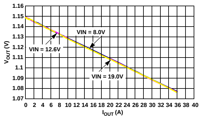
FIGURE 5. ACTIVE MODE LOAD LINE, 2 PHASE, CCM, \text{PSI}_L = \text{HIGH} , \text{VID} = 1.15\text{V}
