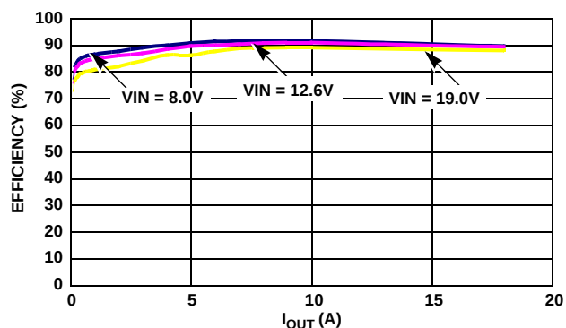
FIGURE 6. ACTIVE MODE EFFICIENCY, 1 PHASE, DE, \text{PSI}_L = \text{LOW} , \text{VID} = 1.15\text{V}
