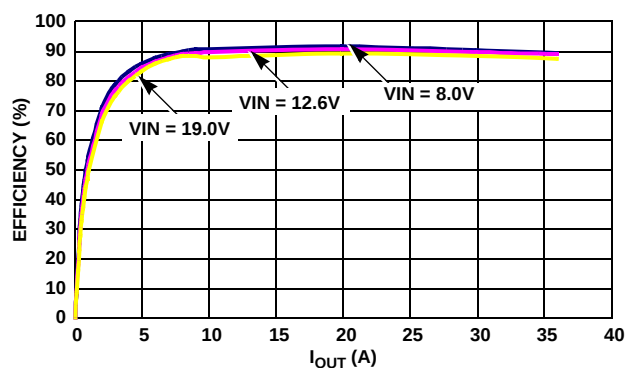
FIGURE 4. ACTIVE MODE EFFICIENCY, 2 PHASE, CCM, \text{PSI}_L = \text{HIGH} , \text{VID} = 1.15\text{V}
