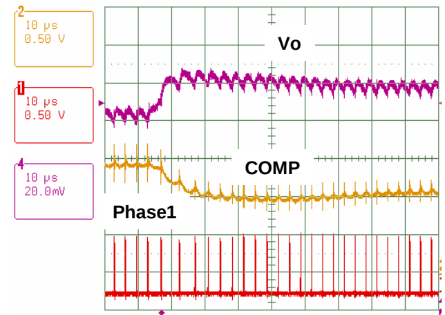
FIGURE 19. LOAD RELEASE RESPONSE AT 1-PHASE DE MODE, ILOAD = 19A→4A, PSI L = 0, AND VID = 1V
