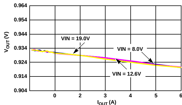
FIGURE 9. 1-PHASE DE MODE LOAD LINE, \text{PSI}_L = \text{LOW} , \text{VID} = 0.9\text{V} , \text{OFFSET} = 33\text{mV}
