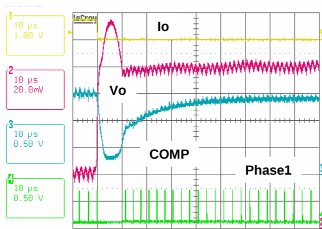
FIGURE 17. LOAD RELEASE RESPONSE AT 2-PHASE CCM, VIN = 19V, ILOAD = 46A→10A, AND VID = 1.15V
