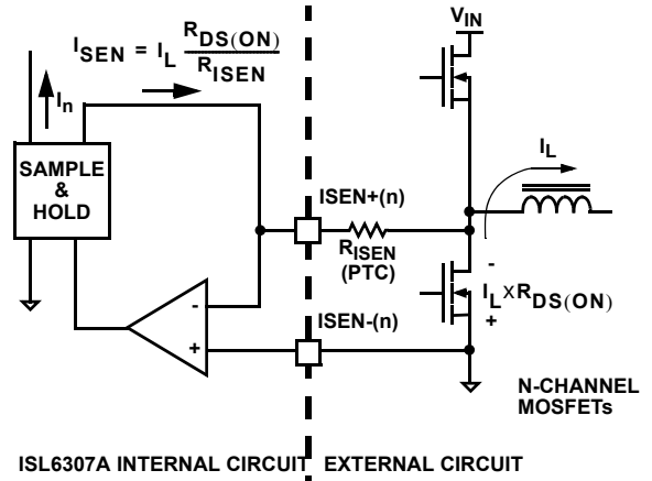
FIGURE 6. MOSFET R_{DS(ON)} CURRENT-SENSING CIRCUIT
