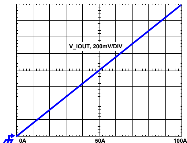
FIGURE 17. VOLTAGE AT IOUT PIN WITH A RESISTOR TO GND WHEN LOAD CURRENT CHANGES
