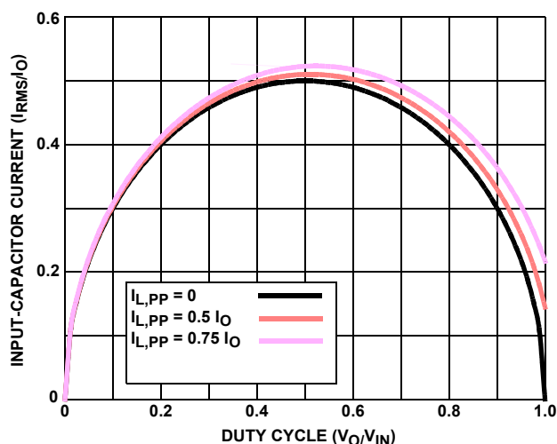
FIGURE 28. NORMALIZED INPUT-CAPACITOR RMS CURRENT vs DUTY CYCLE FOR SINGLE-PHASE CONVERTER
