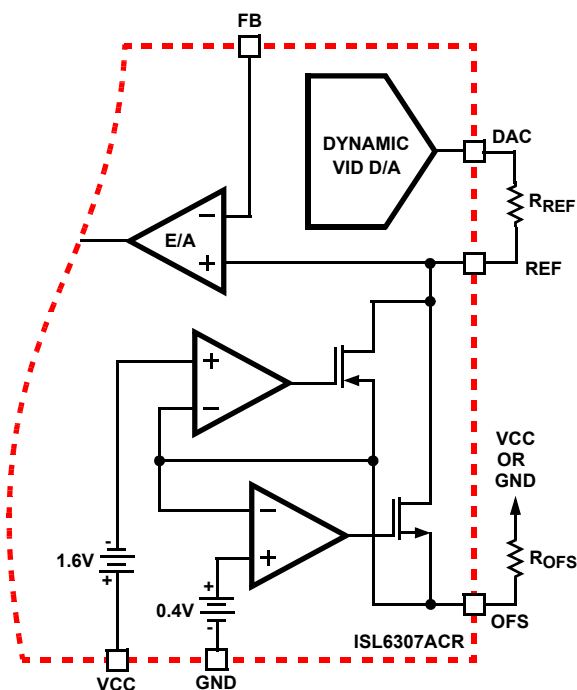
FIGURE 9. OUTPUT VOLTAGE OFFSET PROGRAMMING WITH ISL6307A
