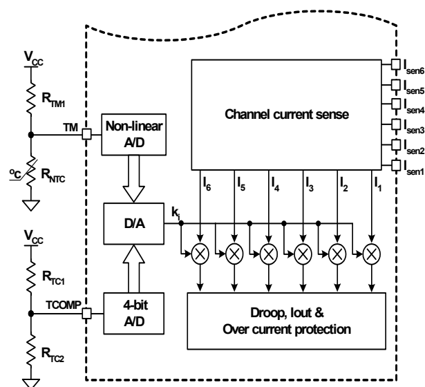
FIGURE 21. BLOCK DIAGRAM OF INTEGRATED TEMPERATURE COMPENSATION
