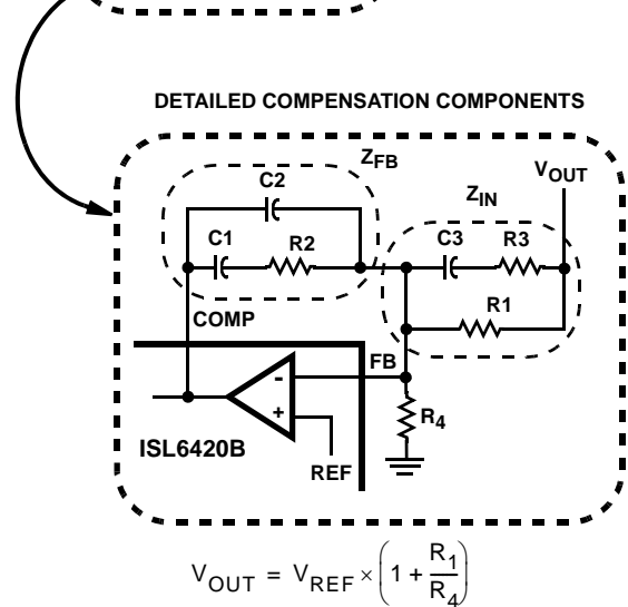
FIGURE 17. VOLTAGE - MODE BUCK CONVERTER COMPENSATION DESIGN
