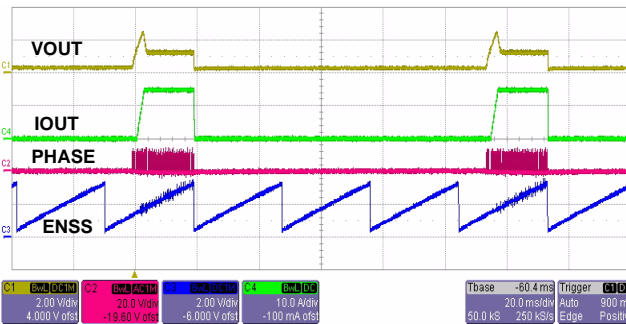
FIGURE 10. TYPICAL OVERCURRENT HICCUP MODE
