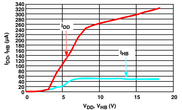
FIGURE 20. ISL89401 QUIESCENT CURRENT vs VOLTAGE
