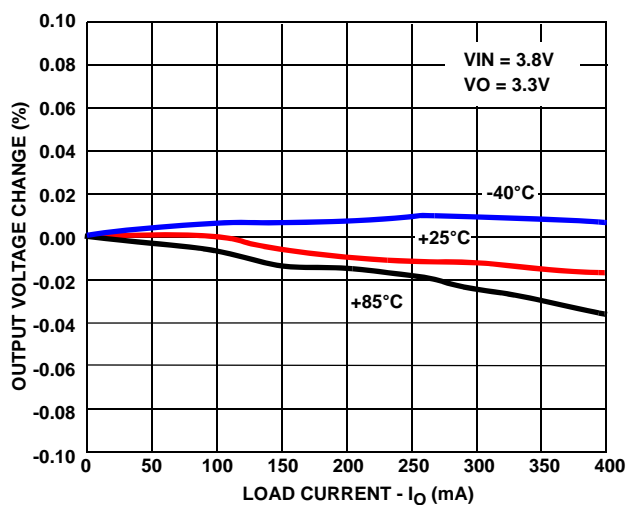
FIGURE 3. OUTPUT VOLTAGE CHANGE vs LOAD CURRENT
