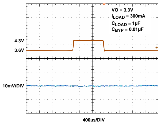
FIGURE 15. LINE TRANSIENT RESPONSE (3.3V OUTPUT)
