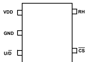
ISL90460 (5 LD SOT-23, SC-70) TOP VIEW
