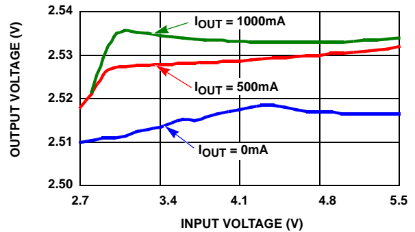
FIGURE 8. V_{OUT} vs V_{IN} (MODE = V_{IN} , V_{OUT} = 2.5V )
