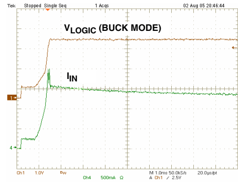
FIGURE 14. I_{IN} RUSH CURRENT
