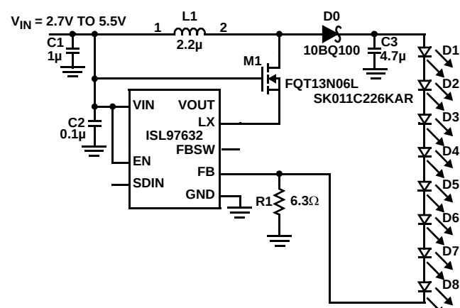
FIGURE 9. CONCEPTUAL 8 LEDs HIGH VOLTAGE DRIVER
