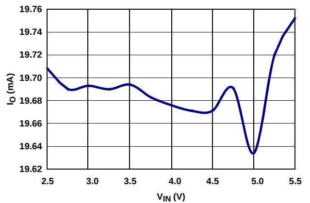
FIGURE 5. LINE REGULATION
