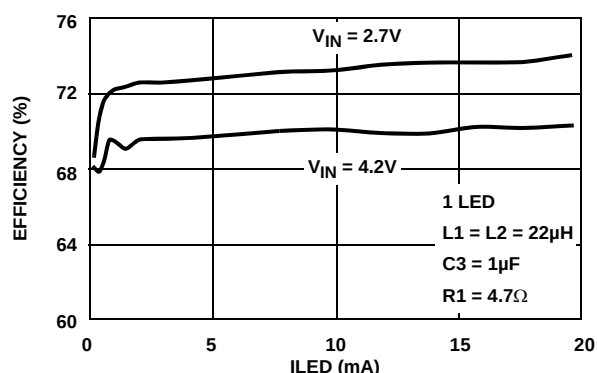
FIGURE 11. EFFICIENCY MEASUREMENT OF A SINGLE LED SEPIC DRIVER
