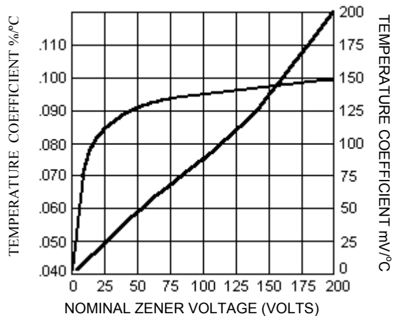
FIGURE 2 ZENER VOLTAGE TEMPERATURE COEFFICIENT vs. ZENER VOLTAGE
