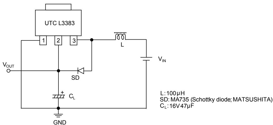
Fig.1 3-Lead Package Application(SOT-89)
