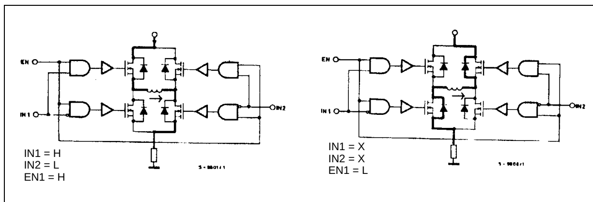
Figure 5. Enable Chopping
