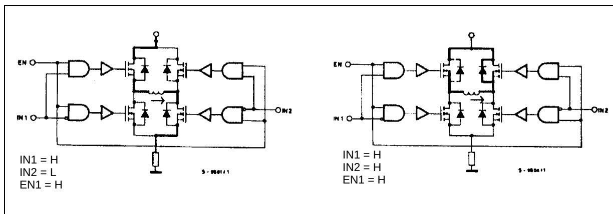
Figure 5. Enable Chopping
