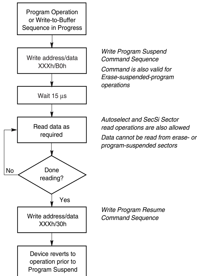
Figure 6. Program Suspend/Program Resume
