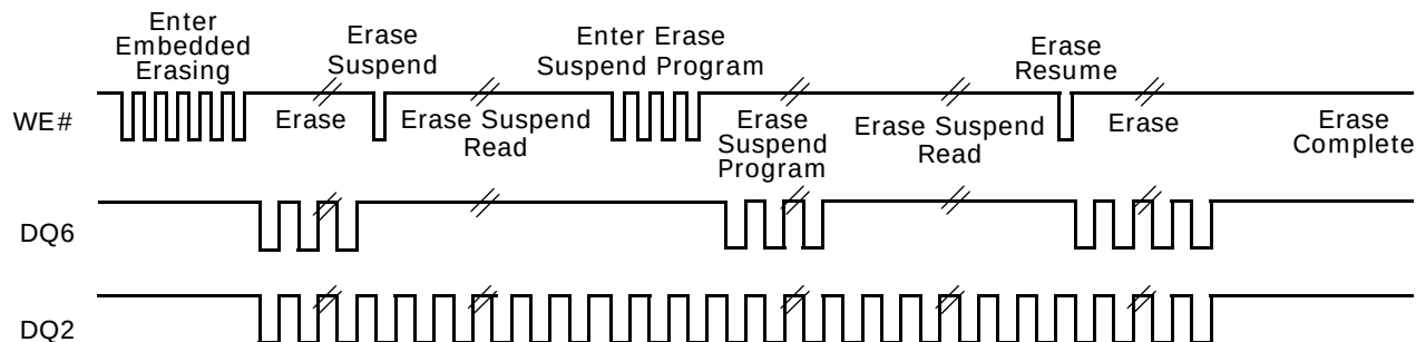
Figure 21. Toggle Bit Timings (During Embedded Algorithms)
