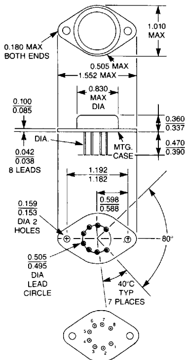
Bottom View
