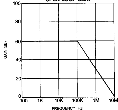
ERROR AMPLIFIER OPEN LOOP GAIN
