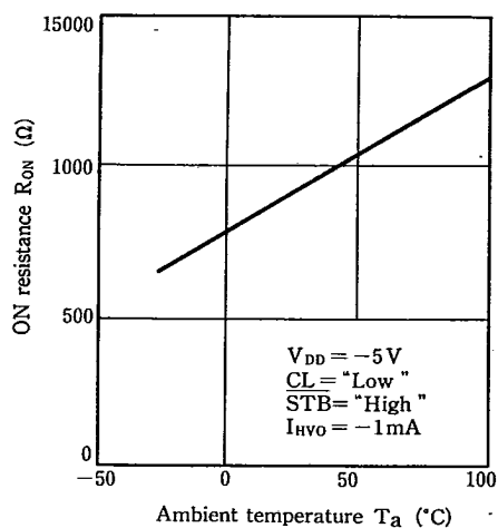
ON resistance vs. Ambient temperature
