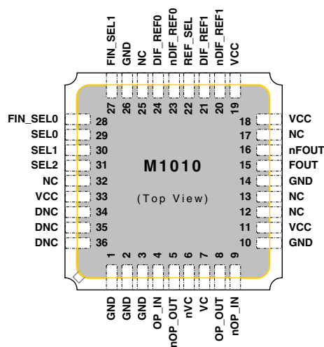
Figure 1: Pin Assignment
