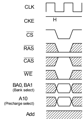
Fig. 3 Precharge command
