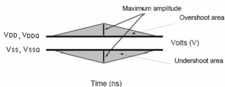
Overshoot/Undershoot Definition
