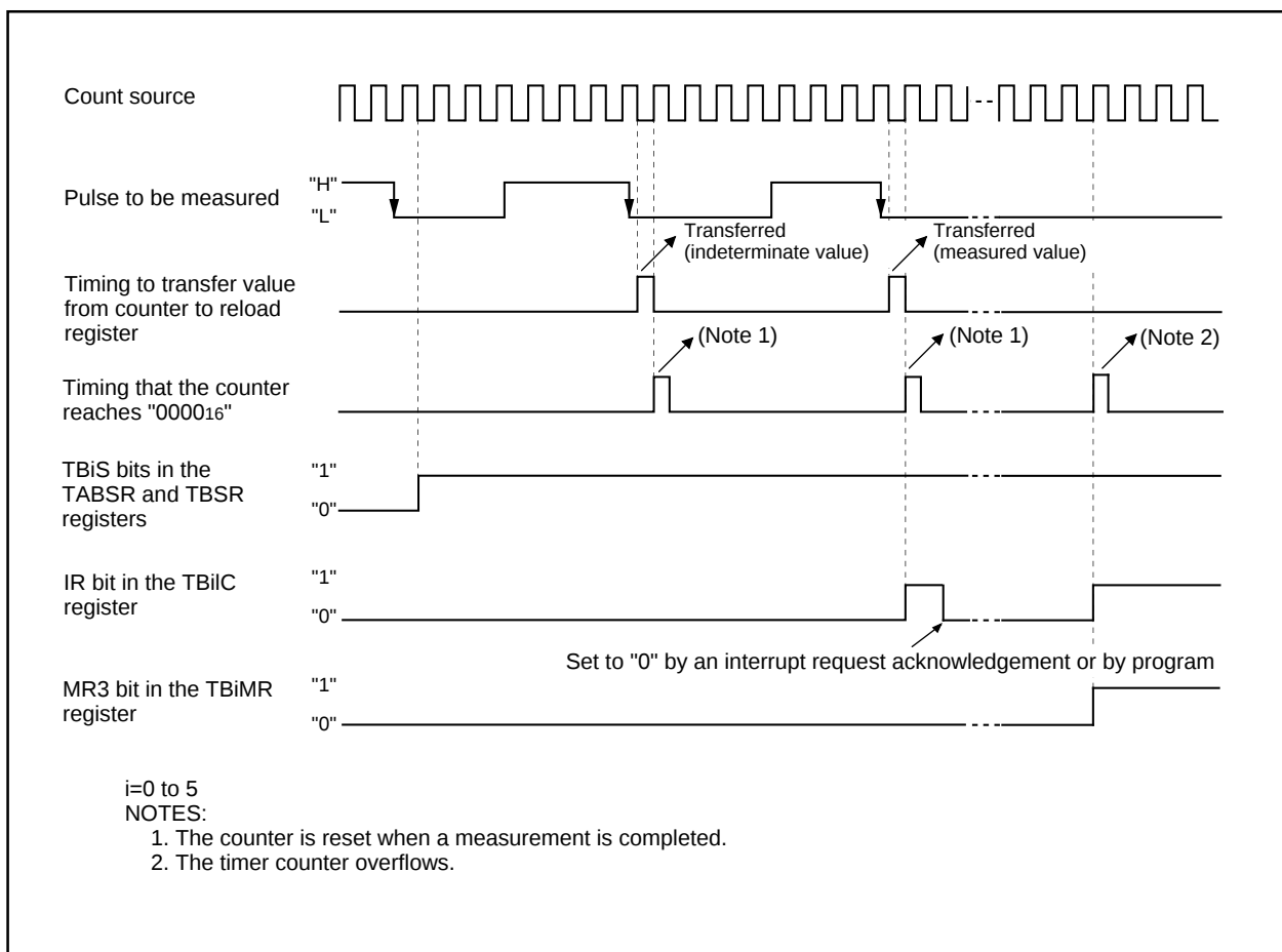
Figure 14.23 Operation Example in Pulse Period Measurement Mode
