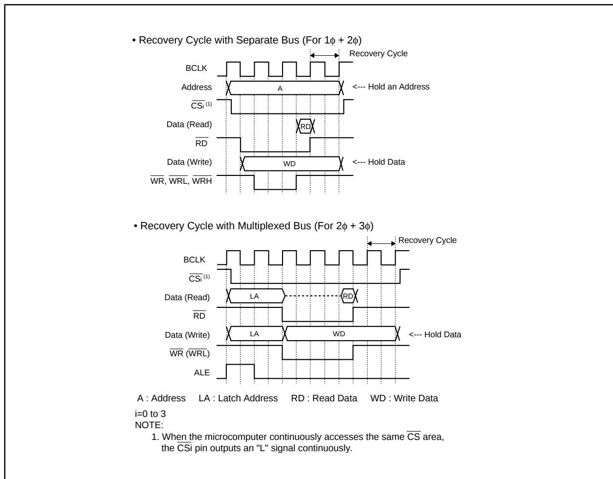
Figure 7.9 Recovery Cycle
