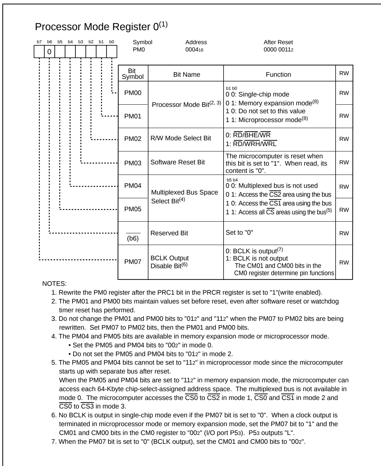
Figure 6.1 PM0 Register
