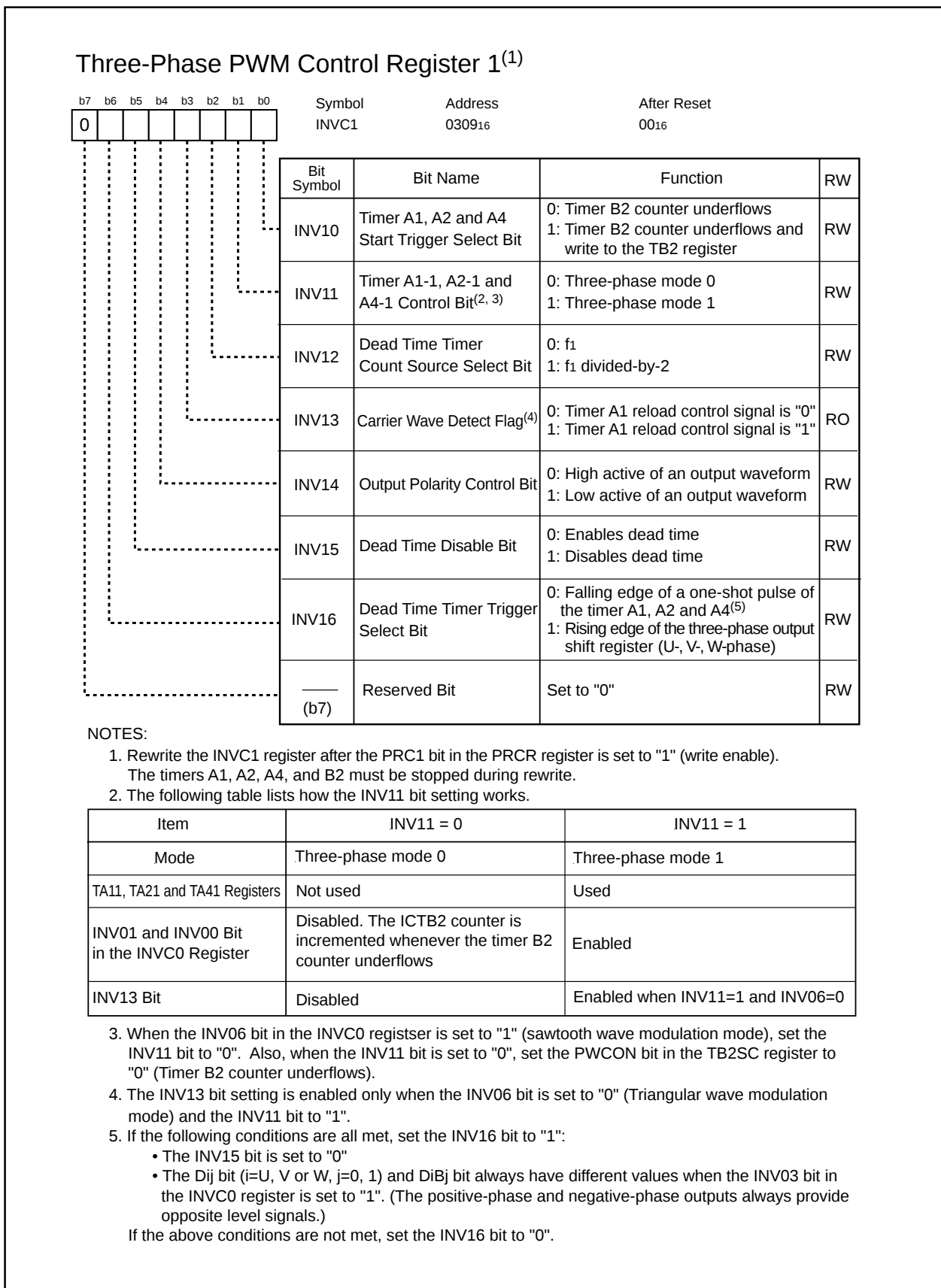
Figure 15.3 INVC1 Register
