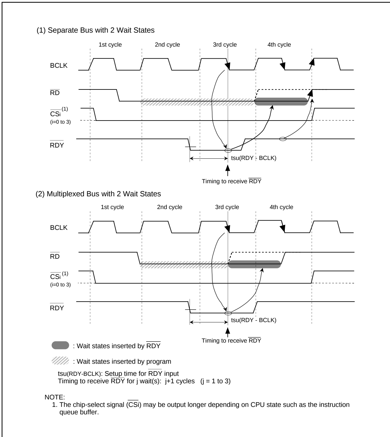
Figure 7.11 \overline{\text{RD}} Signal Output Extended by \overline{\text{RDY}} Signal
