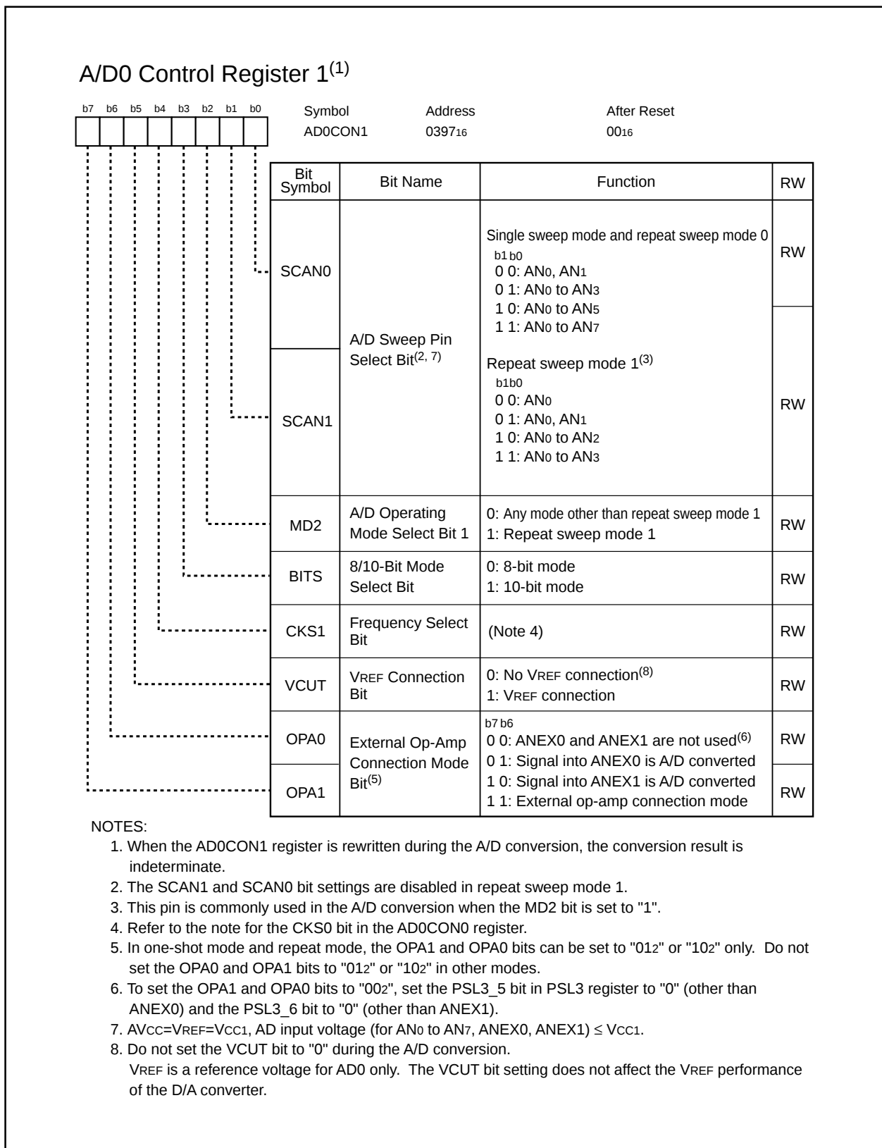
Figure 17.3 AD0CON1 Register
