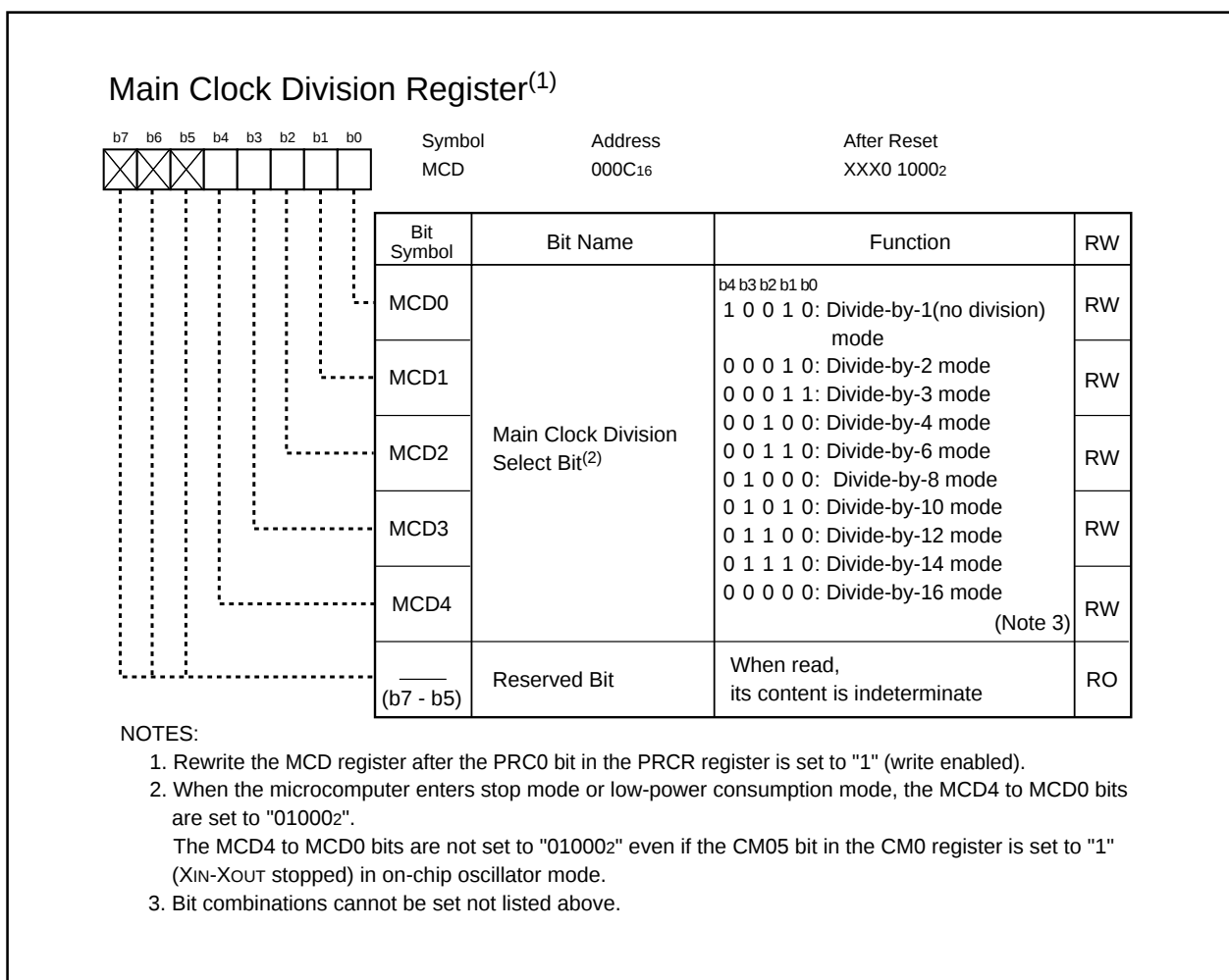
Figure 8.4 MCD Register
