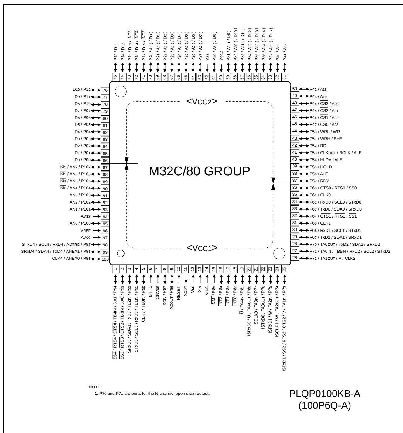
Figure 1.4 Pin Assignment
