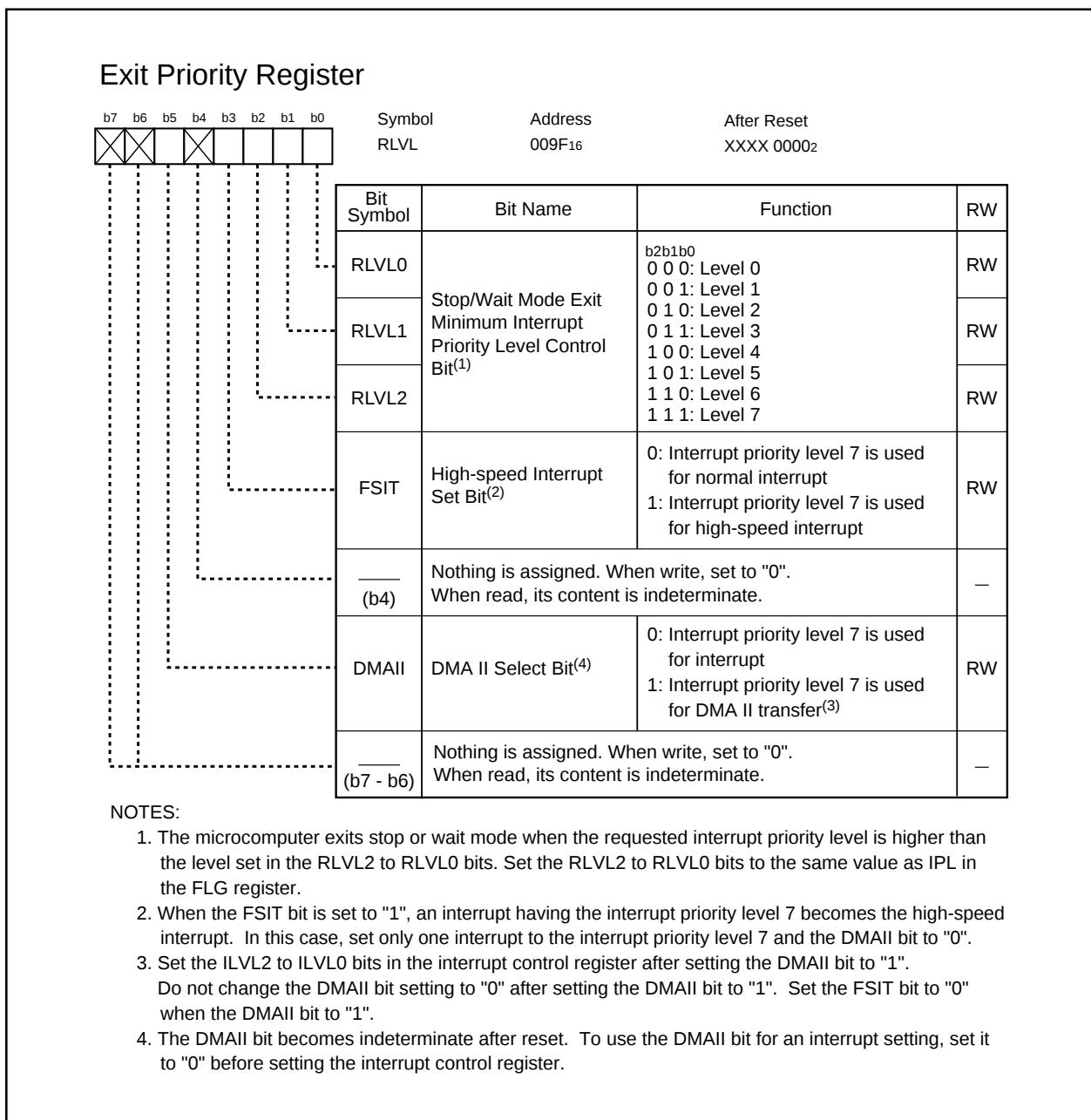
Figure 10.5 RLVL Register
