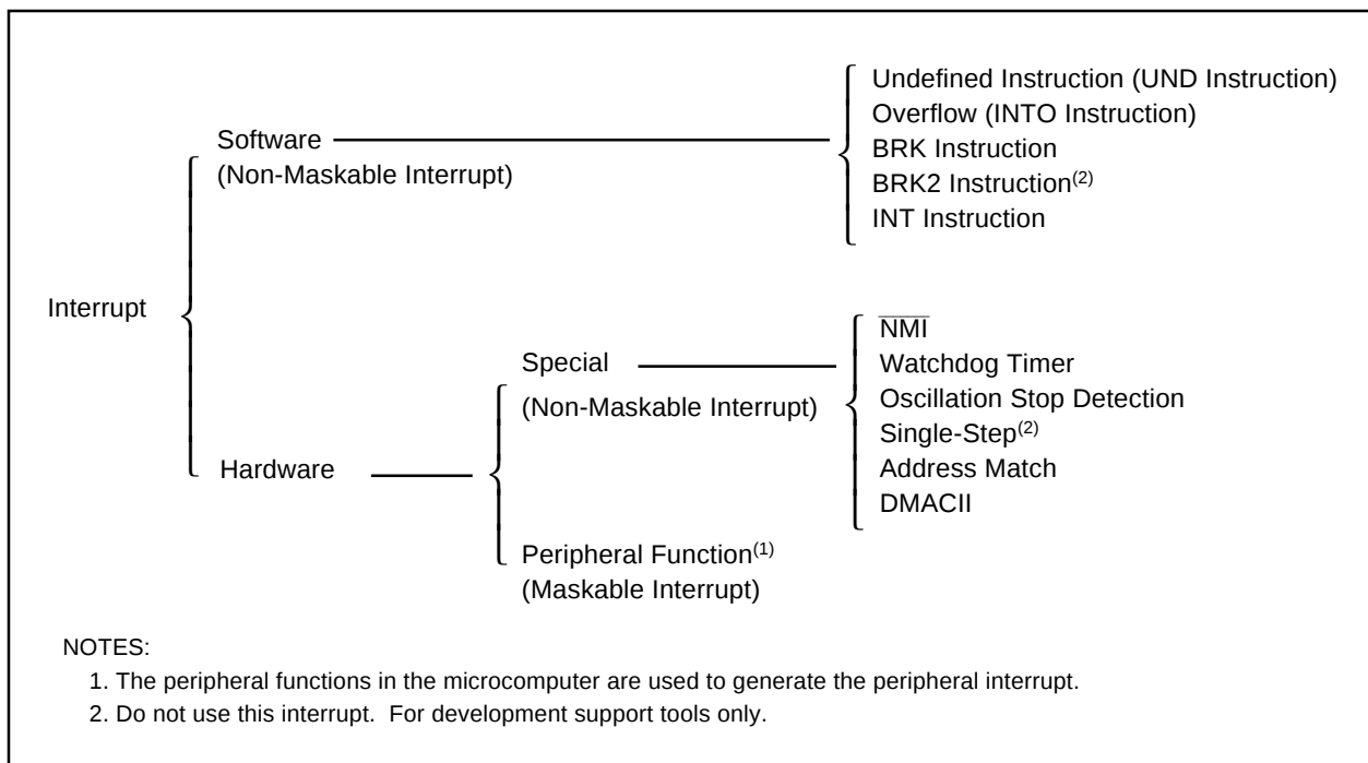
Figure 10.1 Interrupts
