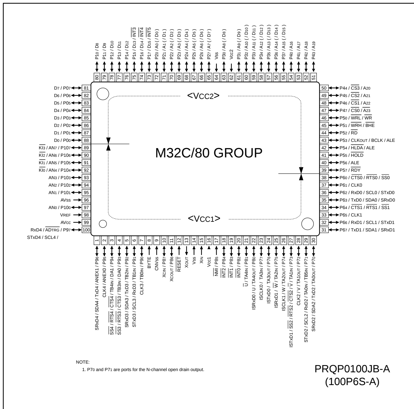
Figure 1.3 Pin Assignment
