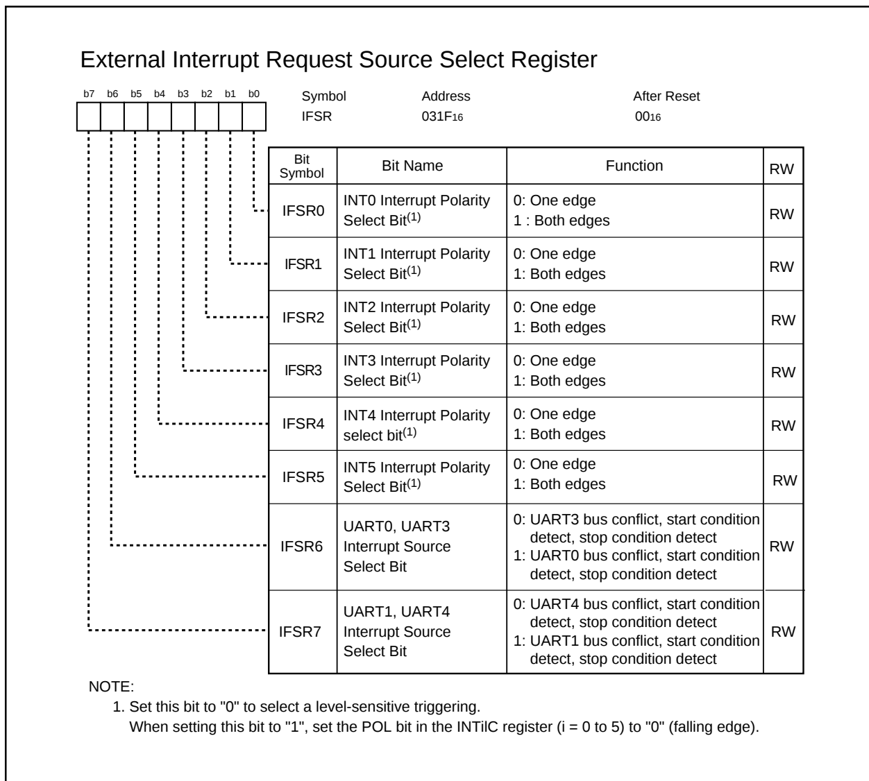
Figure 16.9 IFSR Register
