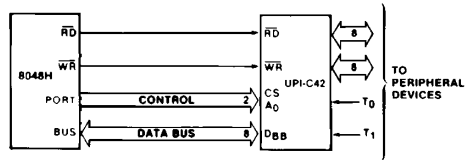
Figure 9. 8048H-UPI-C42 Interface
