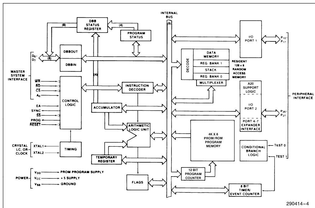
Figure 4. Block Diagram
