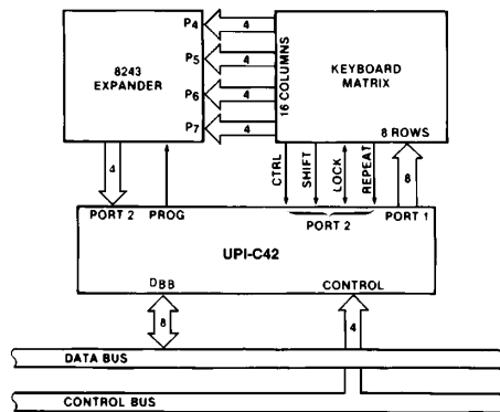
Figure 10. UPI-C42-8243 Keyboard Scanner
