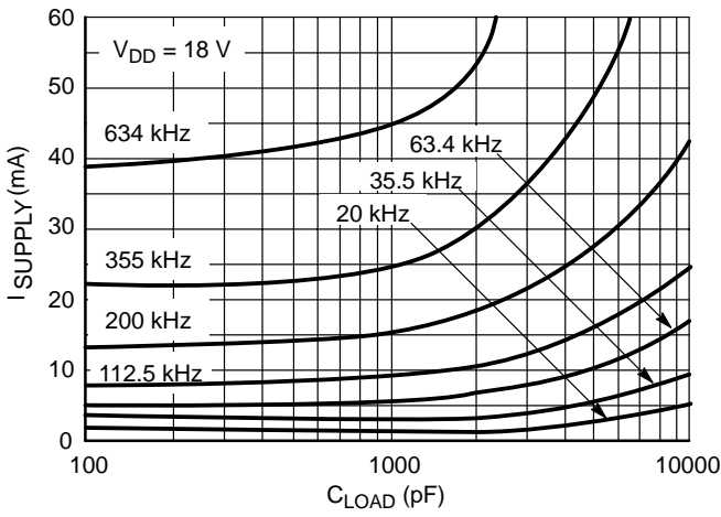
Figure 15. Supply Current vs. Capacitive Load
