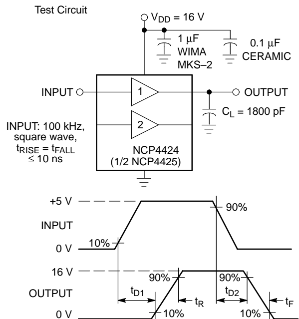
Figure 2. Noninverting Driver Switching Time
