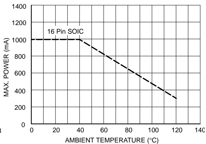
Figure 22. Thermal Derating Curves
