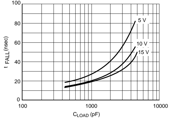
Figure 6. Fall Time vs. Capacitive Load
