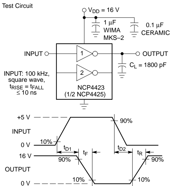
Figure 1. Inverting Driver Switching Time
