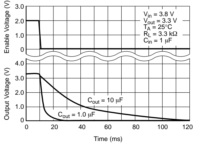
Figure 23. Turn-off Response
