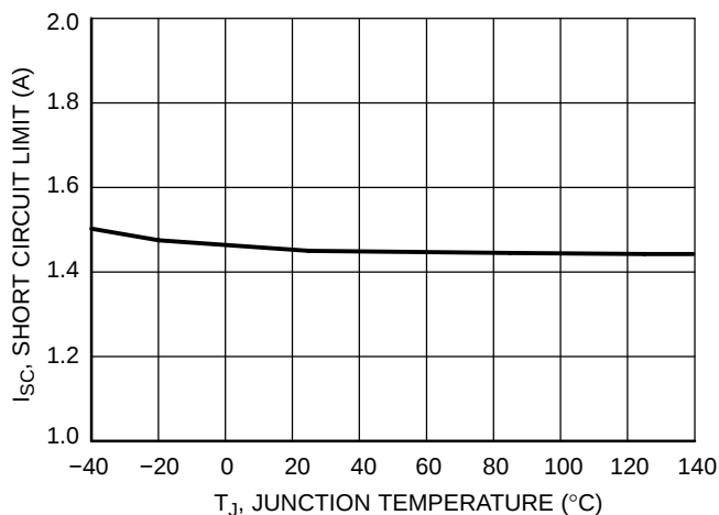
Figure 6. Short Circuit Current Limit vs. Temperature
