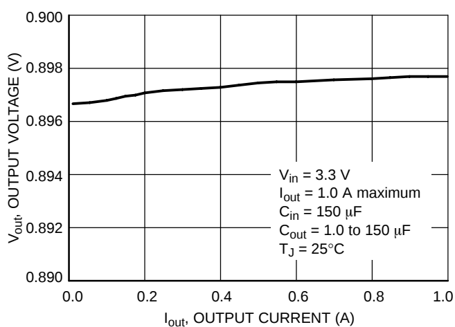
Figure 8. Output Voltage vs. Output Load Current
