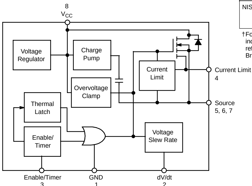
Figure 1. Block Diagram
