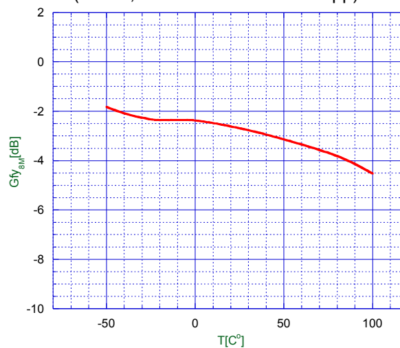
LPF Characteristics vs. Temperature ( V^+=3V , v_{in}=8MHz/100kHz 0.5Vpp)
