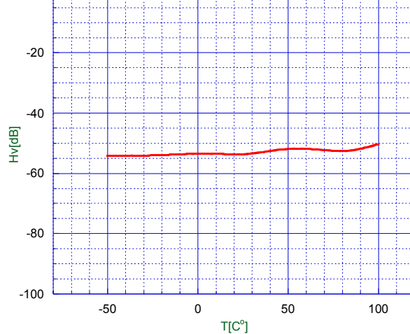
2 nd Distortion vs. Temperature ( V^+=3V , R_L=75ohm , v_{in}=0.5Vpp 3.58MHz sine-signal)
