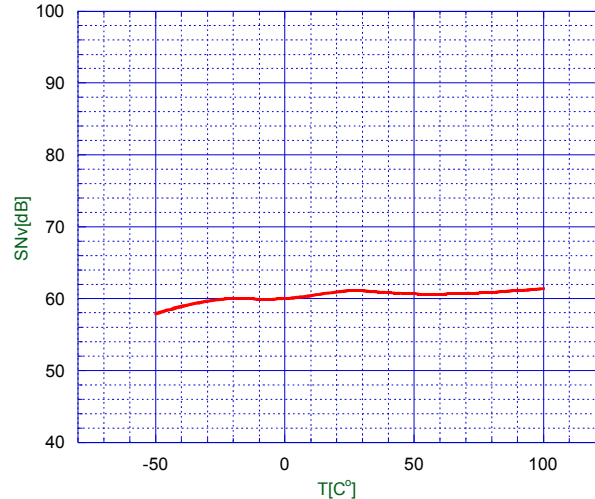
S/N Ratio vs. Temperature ( V^+=3V , R_L=75ohm , v_{in}=0.5Vpp White Video Signal 100kHz to 6MHz)
