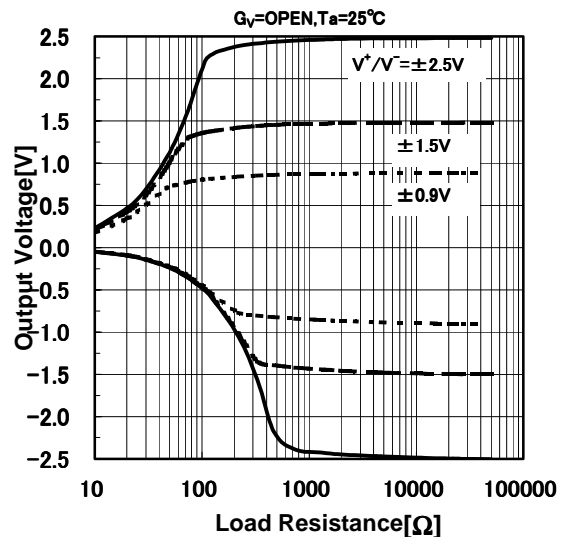
Output Voltage vs. Load Resistance ( V^+/V^- )
