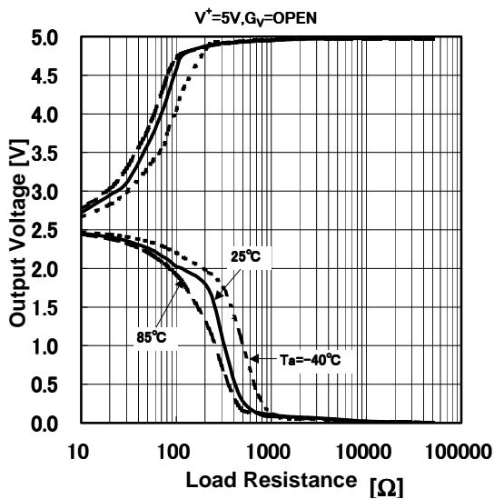
Output Voltage vs. Load Resistance (Temp.)
