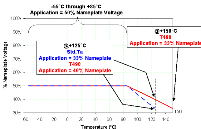
Figure 5. Recommended application voltages versus temperature.
