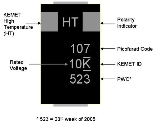
Figure 3. Component marking diagram for T498 capacitor.
