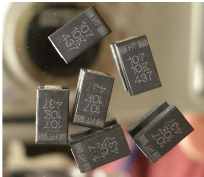
Figure 2. Photograph of "D" case, T498 SMT capacitors.
